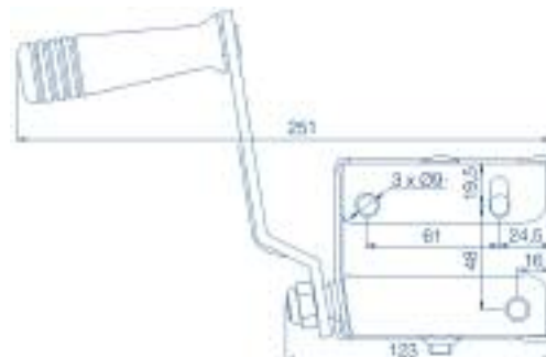
Base Mounting
